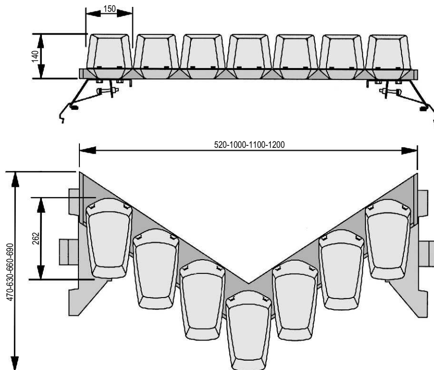
Vector Series lightbar. Dimensions (mm)
